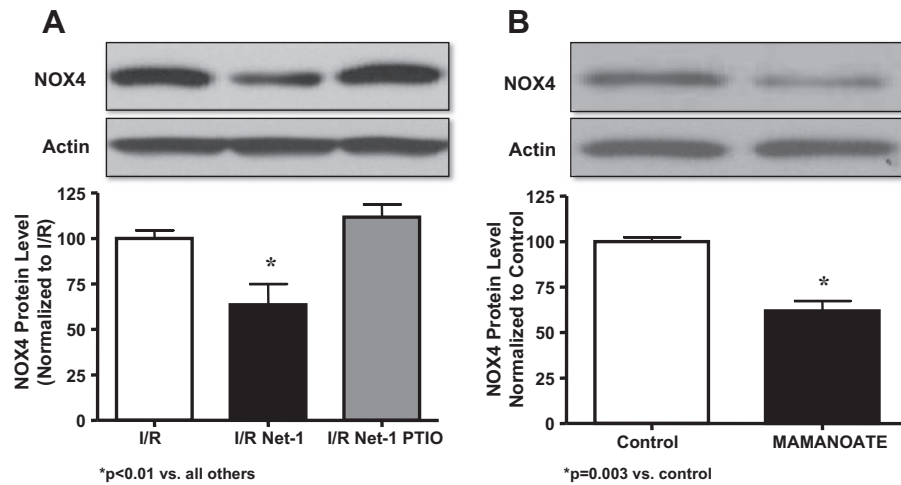
Fig. 2. Nitric oxide (NO) mediates netrin-1 downregulation of NOX4 protein abundance. A) NOX4 protein level in I/R injured hearts that were subjected to netrin-1 with or without NO scavenger PTIO. The reduction in NOX4 protein level in netrin-1 treated hearts was abolished by co-treatment with PTIO ( p < 0.01 vs. all others, n = 3 ). B) NOX4 protein level in freshly isolated adult cardiomyocytes was significantly downregulated by the NO donor MAMANOATE (1 mmol/L) ( p = 0.003 vs. control, n = 3 ).
