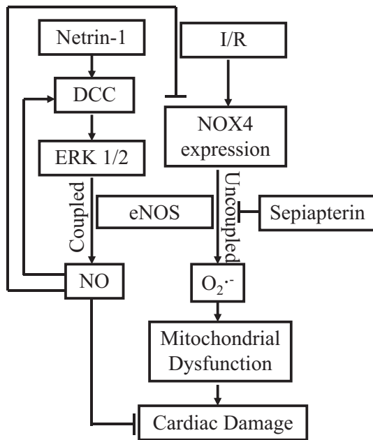
Fig. 5. Molecular mechanisms underlying netrin-1 induced cardioprotection. Netrin-1 perfusion activates its transmembrane receptor DCC, leading to ERK-dependent activation of eNOS phosphorylation and NO production, which in turn exerts direct cardioprotective effects that are NO-mediated. On the other hand, netrin-1 derived NO attenuates I/R activation of NOX4, resulting in recoupled NOS, and preserved mitochondrial function. All together, these pathways maintain a positive feed-forward loop of sustained endogenous production of NO, which protects cardiomyocytes against I/R injury to markedly reduce necrosis and apoptosis.
