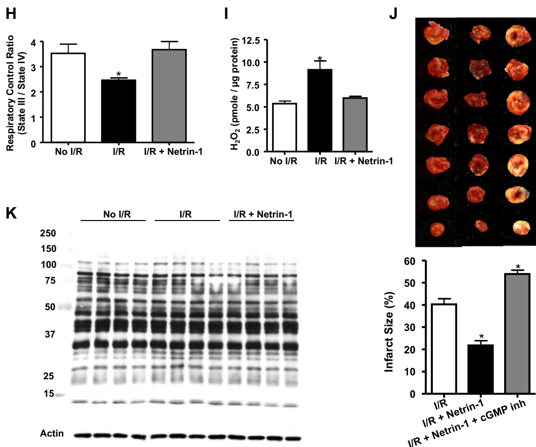
Fig. 1. Netrin-1 attenuates I/R induced increases in superoxide production, NOX activity, NOX4 protein abundance and mitochondrial dysfunction. A) Schematic illustration of experimental protocols. B) Superoxide production from I/R injured hearts with and without netrin-1 perfusion. Superoxide production from heart homogenates was measured using electron spin resonance (ESR), shown as the amount inhibited by Mn-SOD, and normalized to no I/R condition. Superoxide production from the I/R control was significantly higher than all other conditions ( p = 0.001 vs. all others, n = 3 ). Of note, the 2.5-fold increase in superoxide production provoked by I/R was completely attenuated by netrin-1 perfusion. C) NADPH-driven NOX activity assessed using purified membrane fraction of perfused hearts. Measurements shown are superoxide production under control (without addition of NADPH substrate, top), with NADPH (middle), and the difference between the two (bottom), which is an indication of NOX activity. Data indicate that under I/R, NOX activity was significantly increased compared to no I/R, which was completely attenuated by netrin-1 perfusion ( p < 0.001 vs. all others, n = 4 ). D) Western blot showing the specificity of the NOX4 antibody used. NOX4 protein expression was increased in the plasmid overexpressed cells, while decreased in the NOX4 siRNA treated cells. E) Protein levels of NOX1, NOX2 and NOX4 in no I/R, I/R, and netrin-1 perfused I/R-injured hearts. NOX1 and NOX2 protein levels were unchanged. NOX4 was significantly and reproducibly upregulated in I/R-injured hearts, which was abolished by netrin-1 perfusion ( p < 0.001 vs. all others, n = 4 ). F) NOX4 activity assessed using the NOX activity assay with fulvene-5, a specific NOX4 inhibitor. Data show that NOX4 activity was significantly increased by I/R, and reduces to baseline with netrin-1 perfusion ( p < 0.05 , n = 3 ). G) Mitochondrial swelling assay from I/R-injured hearts with or without netrin-1 perfusion. Mitochondrial swelling was measured as an assessment of mitochondrial integrity. Summarized data show that during the monitoring time of 20 min, calcium induced swelling of mitochondria was markedly increased in I/R-injured heart. Perfusion with netrin-1 attenuated this response to baseline ( p < 0.001 vs. all others, n = 4 ). H) Respiratory control ratio, a measure of mitochondrial function, was measured as the ratio of state III (ADP stimulated) versus state IV (oligomycin inhibited) oxygen consumption rate ( n = 4 , p < 0.05 ). I) H_2O_2 as measured with Amplex red ( n = 4 each, p < 0.01 vs all) shows I/R significantly increasing H_2O_2 levels compared with controls, while netrin-1 treatment abolishes this response. J) TTC from I/R-injured hearts after being perfused with netrin-1 or co-perfused with the cGMP inhibitor Rp-8-Br-PET-cGMP ( n = 4 ). The results show that inhibition of cGMP completely eliminated netrin-1's cardioprotective effect. K) Detection of S-nitrosylated proteins from I/R-injured hearts, with or without netrin-1 perfusion. The results show that there were no significant changes in S-nitrosylation of proteins with I/R or perfusion of netrin-1.
