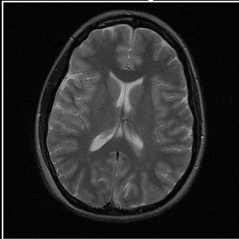
Homodyne
